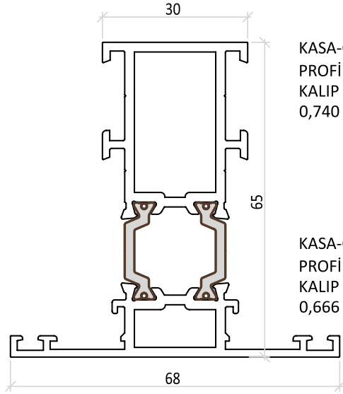
KASA-ORTA KAYIT PROFİLİ KALIP NO 65000 1,406 kg/mt Jx: 28,33 cm 4 Jy: 9,08 cm 4
