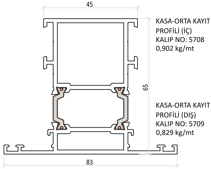
KASA-ORTA KAYIT PROFİLİ KALIP NO 65004 1,732 kg/mt Jx: 35,24 cm 4 Jy: 20,72 cm 4
